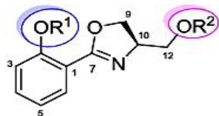
R^1=R^2=H ; Spoxazomicin C 2a: R^1=GI, R^2=H 2b: R^1=GI, R^2=H 2c: R^1=GI, R^2=H
