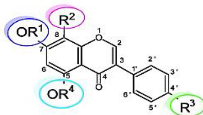
R^1=R^2=H, R^3=OH, R^4=H ; Basic Isoflavonoid 9a: R^1=H, R^2=O(CH_2CH_2)_2NH, R^3=Cl, R^4=Ome 9b: R^1=H, R^2=(CH_2)_5NH, R^3=F, R^4=Ome 9c: R^1=H, R^2=H, R^3=F, R^4=OH 9d: R^1=H, R^2=H, R^3=F, R^4=Ome 9e: R^1=H, R^2=(CH_2)_5NH, R^3=H, R^4=Ome 9f: R^1=H, R^2=O(CH_2CH_2)_2NH, R^3=F, R^4=Ome
